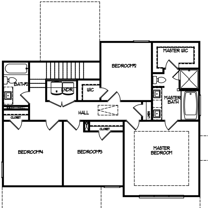
Upper Level
